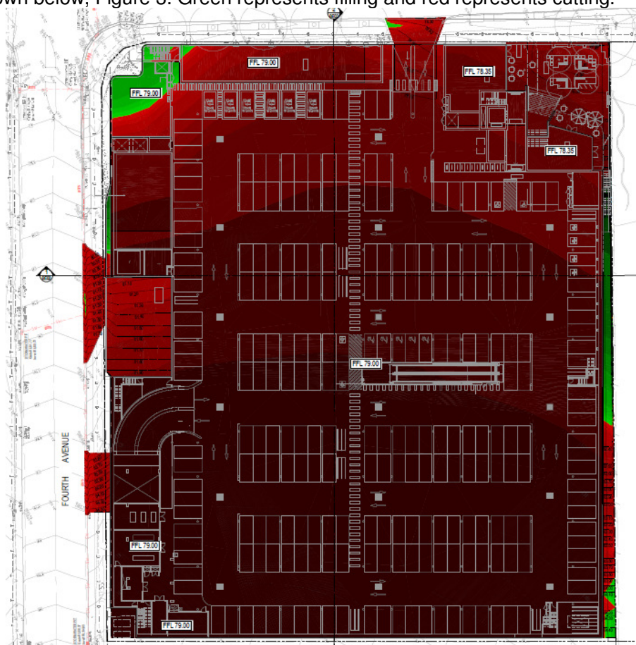
Figure 3: Bulk Earthworks Cut/Fill Plan
